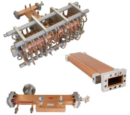
L, S, C-band High Power Ultra High Vacuum Waveguide Components
