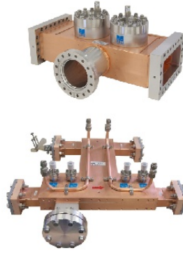
L, S, C-band High Power Ultra High Vacuum Waveguide Components
