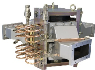
1300MHz WR-650 Waveguide Components
