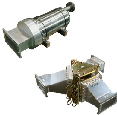
972MHz 3MWpeak WR975 Waveguide Components
